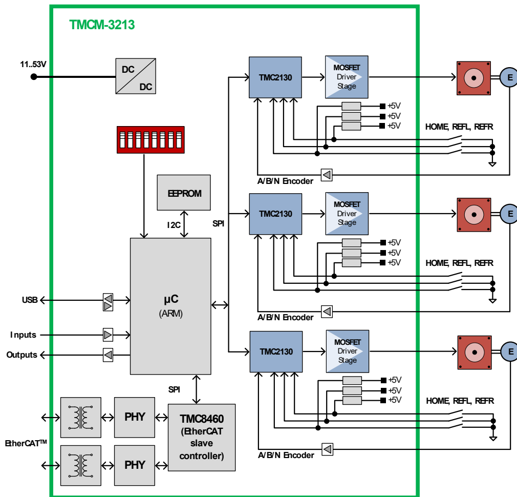
Figure 11.1 Main parts of the TMC3213
