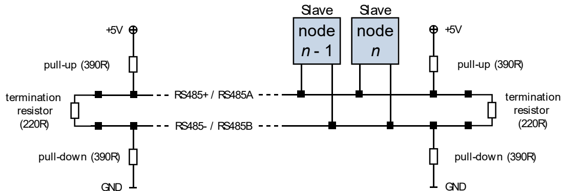
Figure 4.5: Bus lines with resistor (Bias) network at both ends
