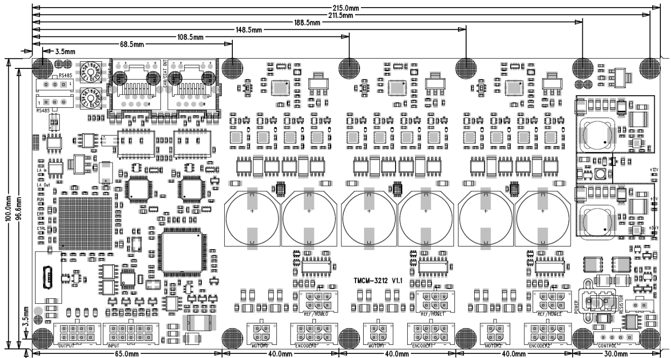
Figure 4.1 Dimension of TMC-3212 / TMC-3213 and position of mounting holes
