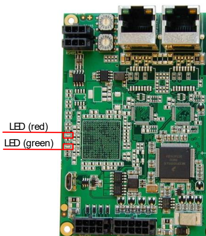
Figure 7.2: LEDs on TMC-3212 interface brick
