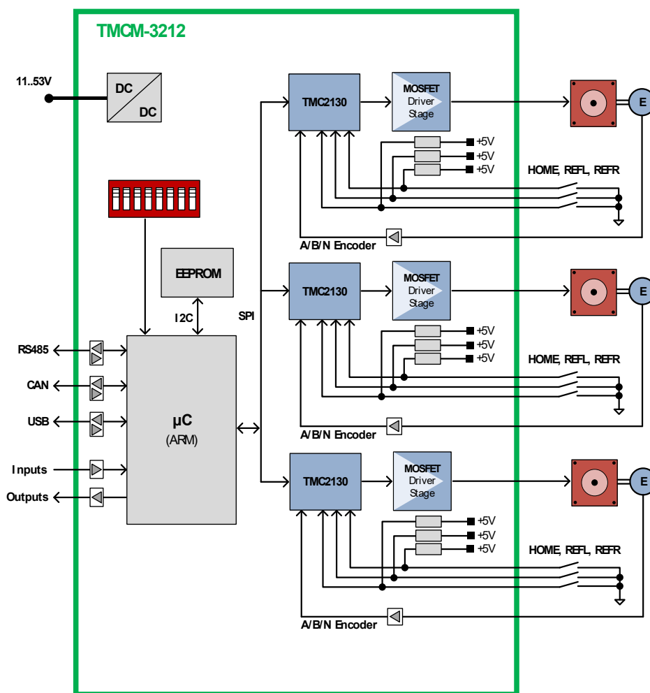
Figure 10.1 Main parts of the TCM-3212
