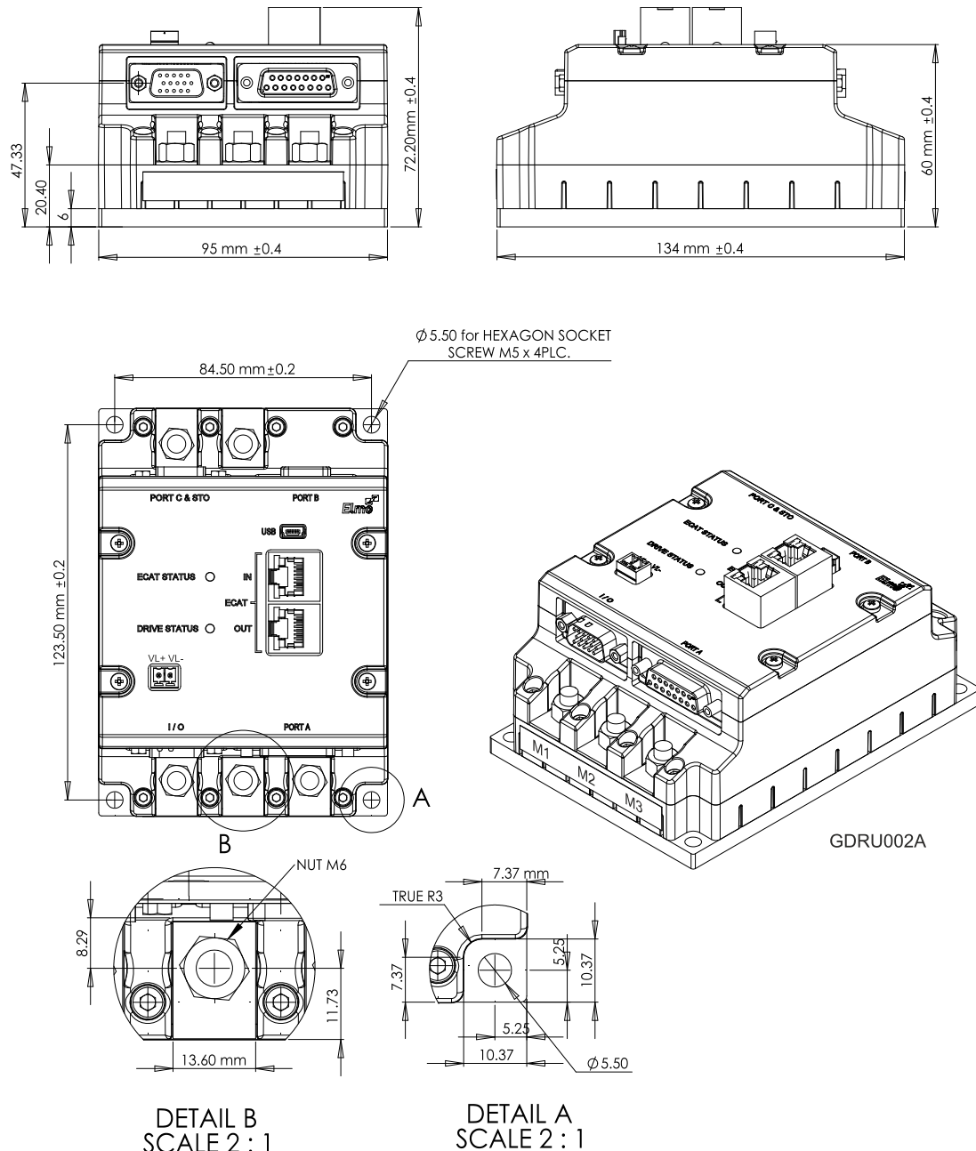
Figure 1: Mounting the Gold Drum with RJ-45 Connectors
